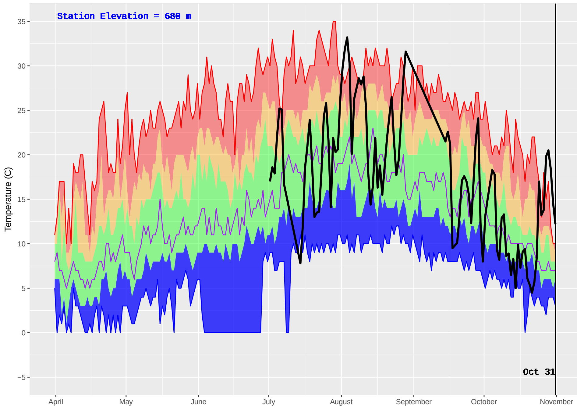
SUMMIT (11) : Historical (1985–2016) and Current (2017) Noon Temperature
