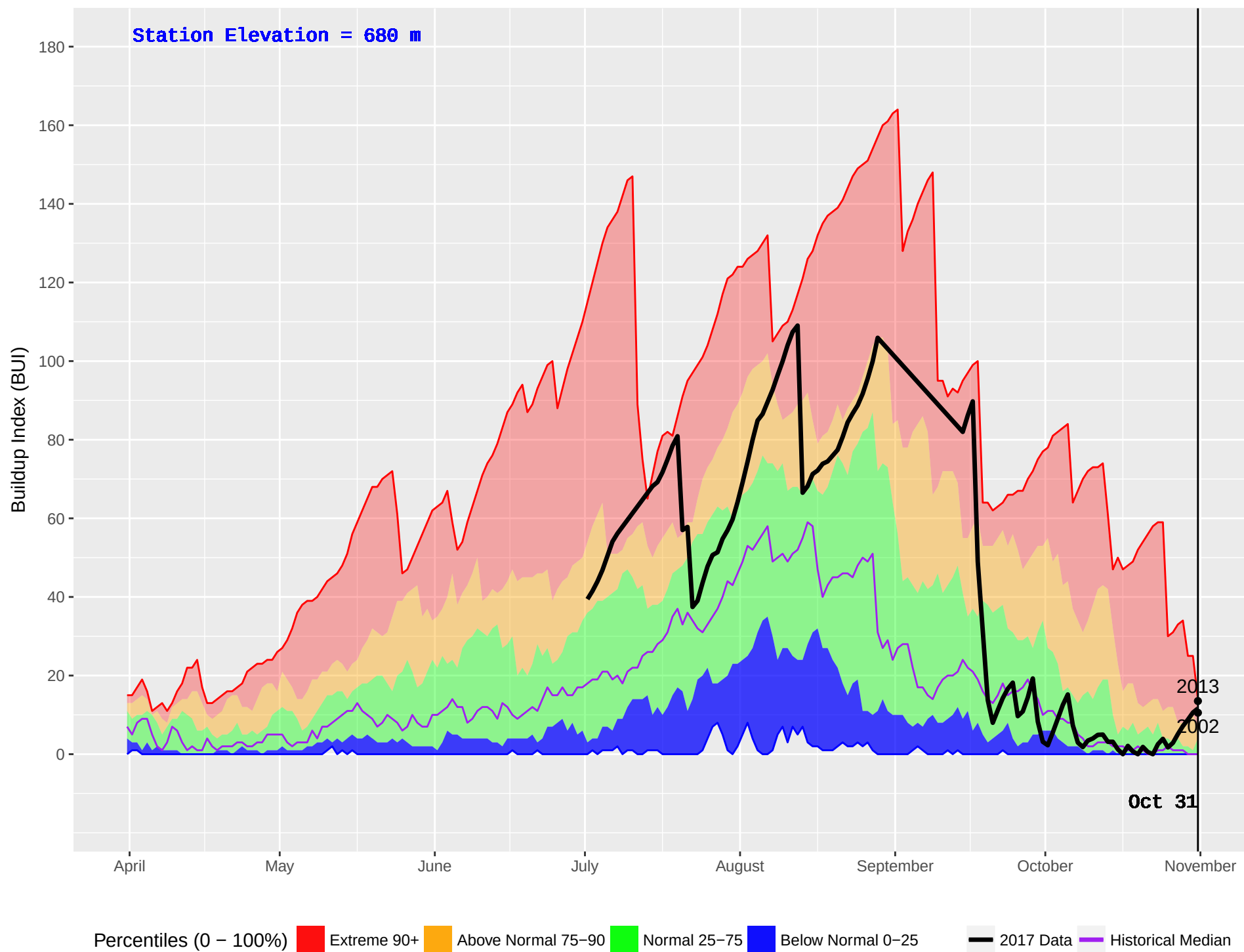
SUMMIT (11) : Historical (1985–2016) and Current (2017) Noon Buildup Index (BUI)
