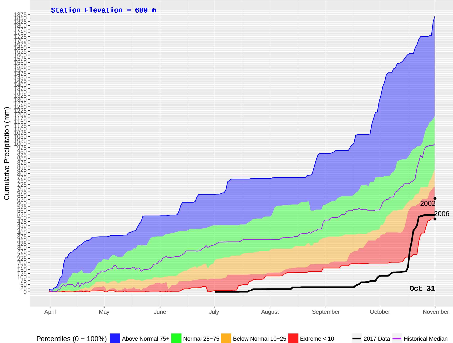
SUMMIT (11) : Historical (1985–2016) and Current (2017) Noon Cumulative Precipitation
