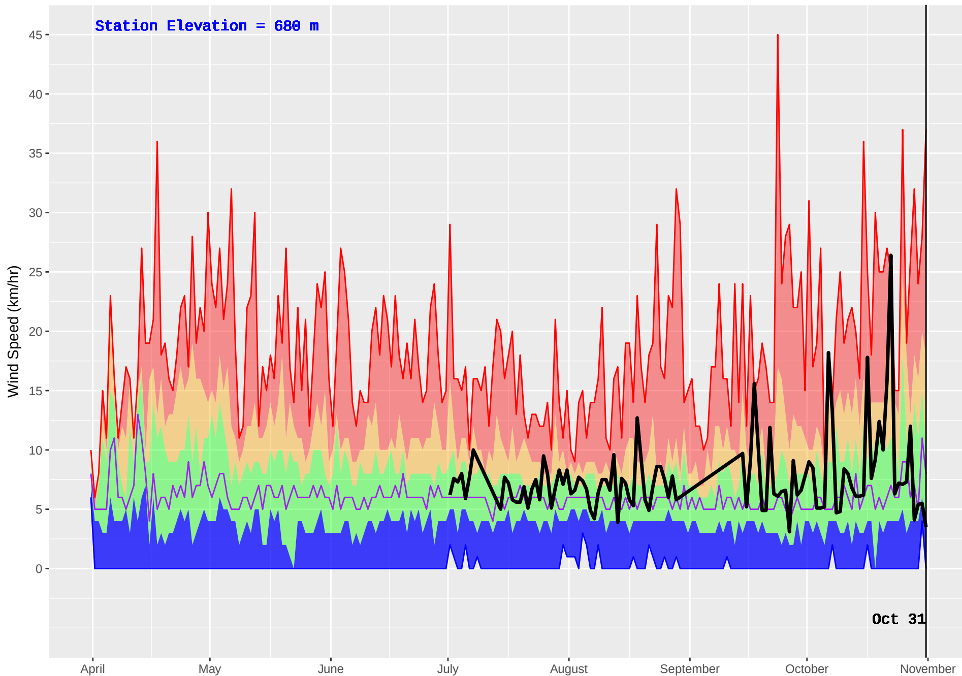
SUMMIT (11) : Historical (1985–2016) and Current (2017) Noon Wind Speed
