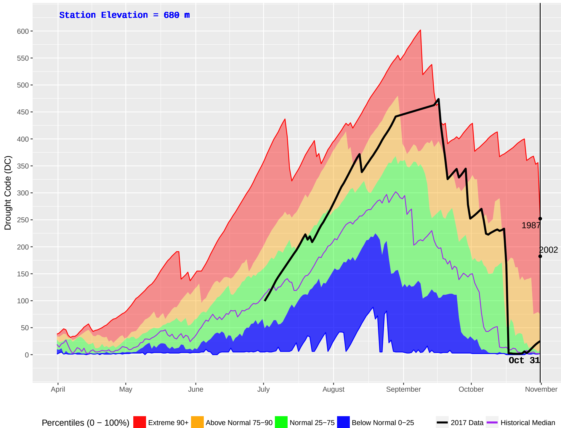
SUMMIT (11) : Historical (1985–2016) and Current (2017) Noon Drought Code (DC)
